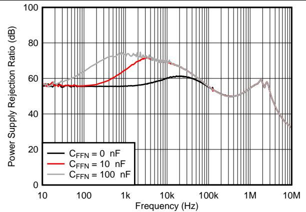
Figure 9. Negative PSRR vs Frequency and C_{FFN}
