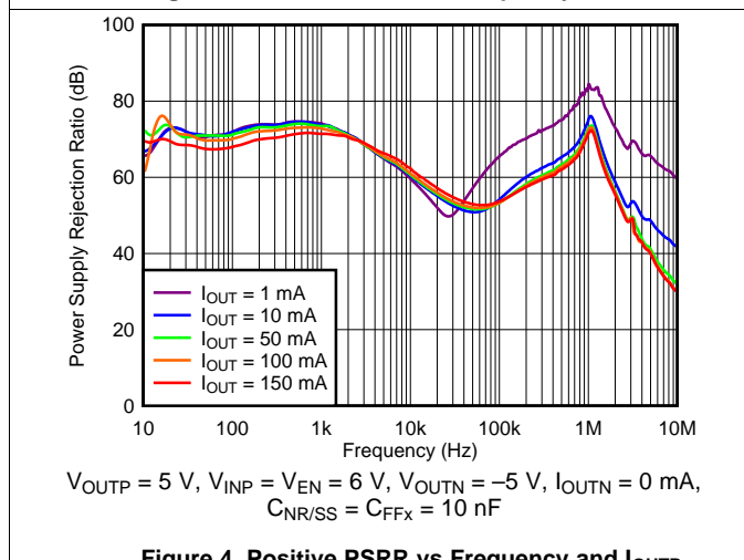
Figure 4. Positive PSRR vs Frequency and I_{OUTP}
