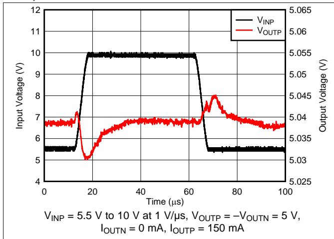
Figure 26. Line Transient Positive Regulator
