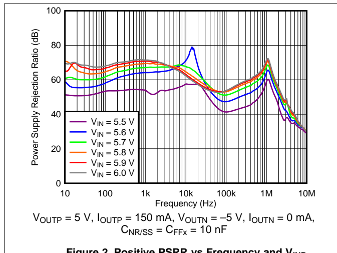
Figure 2. Positive PSRR vs Frequency and V_{INP}
