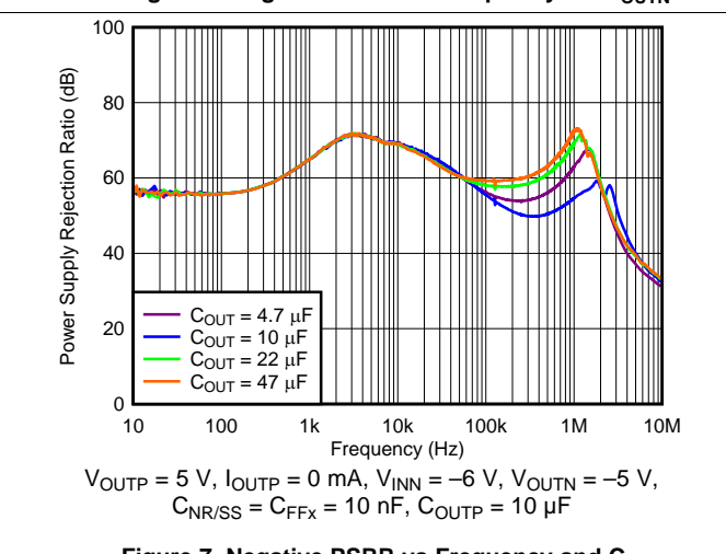
Figure 7. Negative PSRR vs Frequency and C_{OUTN}
