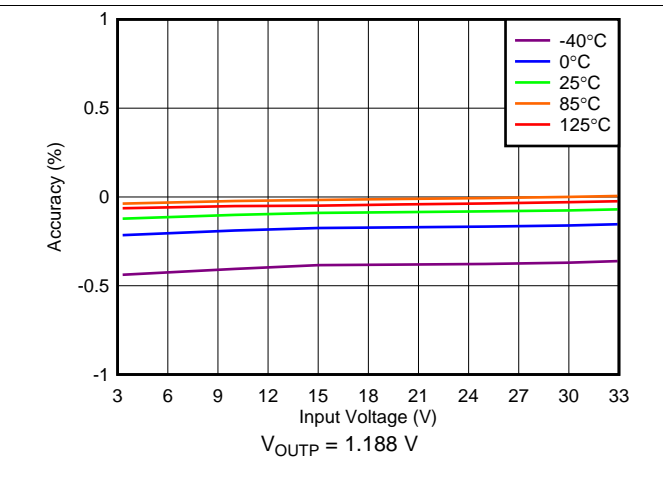
Figure 43. Positive Line Regulation
