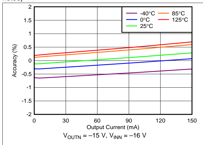
Figure 38. Negative Load Regulation
