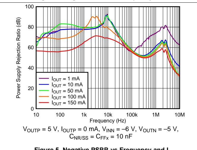
Figure 5. Negative PSRR vs Frequency and I_{OUTN}
