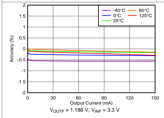
Figure 40. Positive Load Regulation
