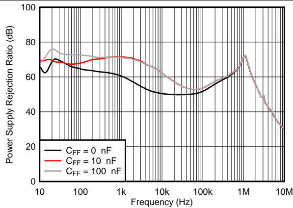
Figure 8. Positive PSRR vs Frequency and C_{FFP}
