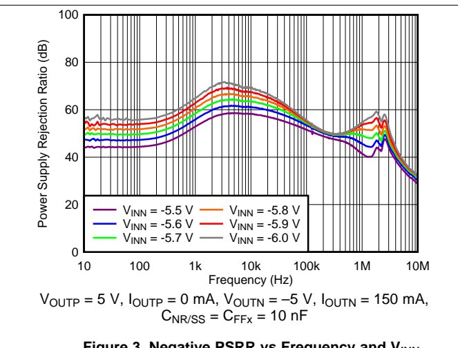
Figure 3. Negative PSRR vs Frequency and V_{INN}
