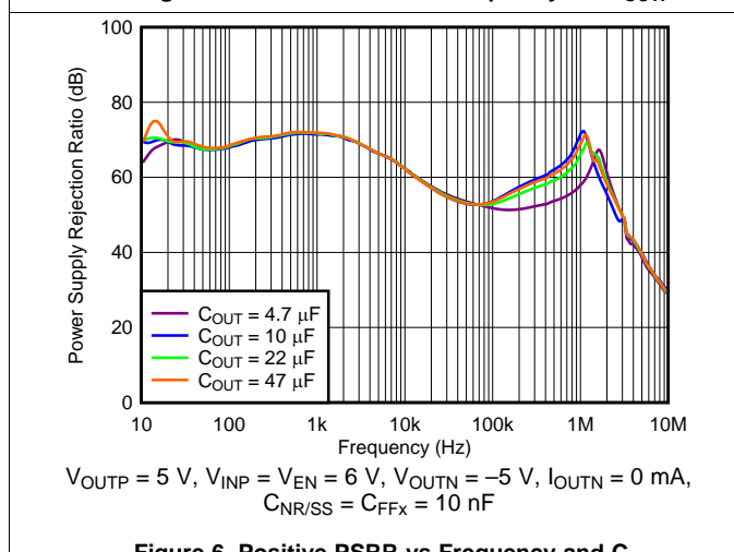
Figure 6. Positive PSRR vs Frequency and C_{OUTP}
