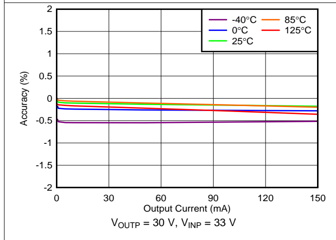
Figure 42. Positive Load Regulation
